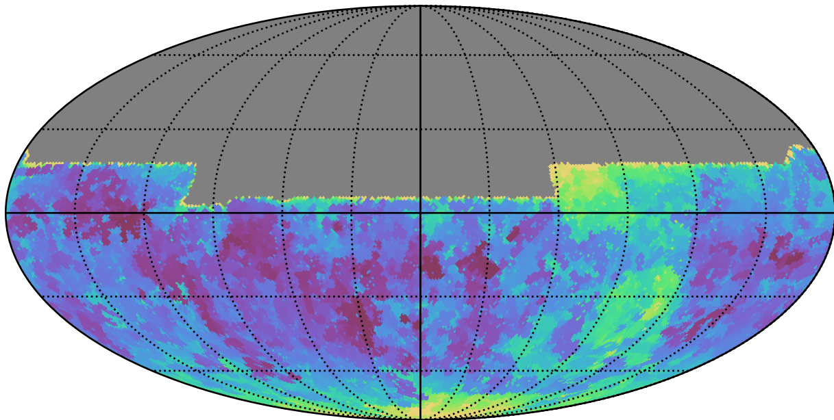
baseline_v2.1_10yrs All sky u band: Min seeingEff
