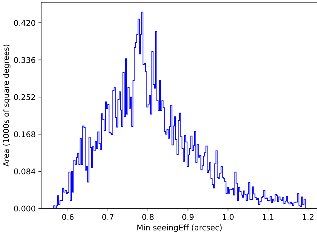
baseline_v2.1_10yrs All sky u band: Min seeingEff
