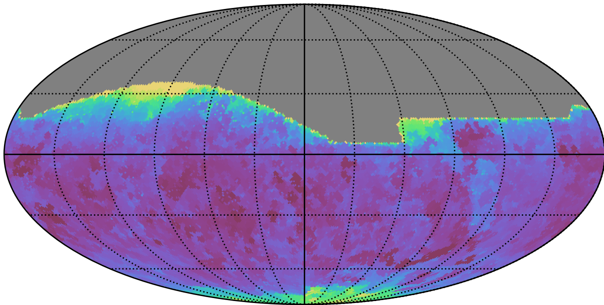
baseline_v2.1_10yrs All sky r band: Min seeingEff
