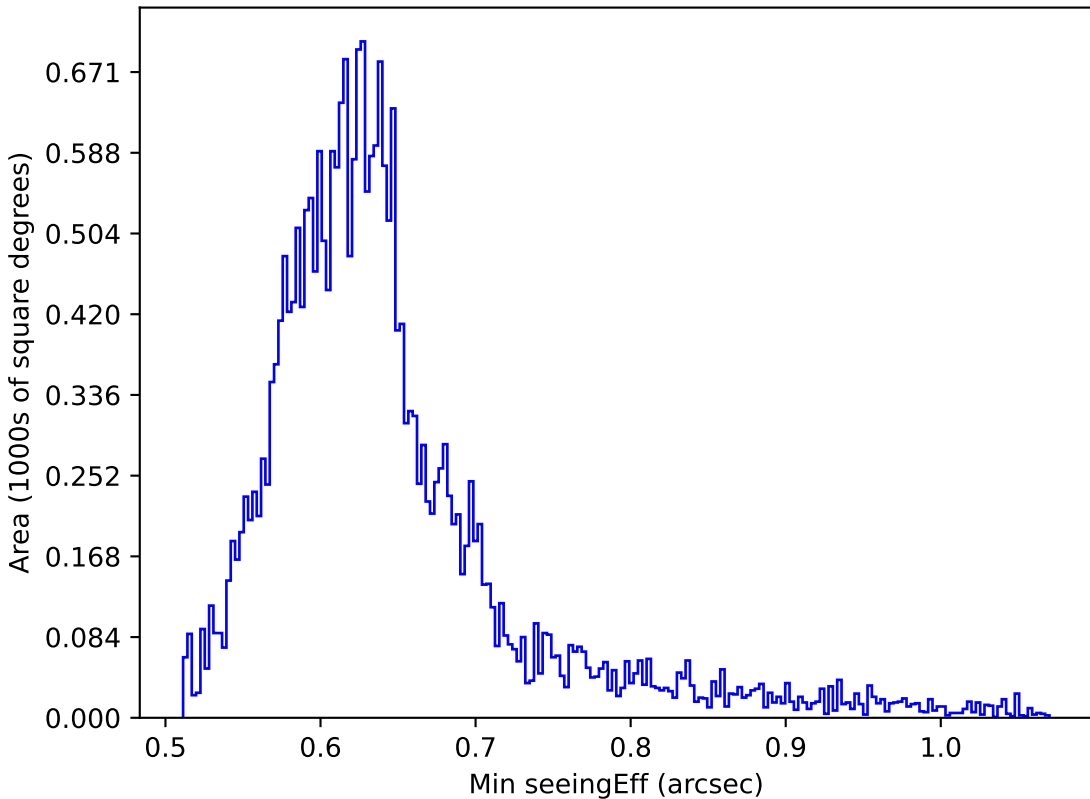
baseline_v2.1_10yrs All sky r band: Min seeingEff
