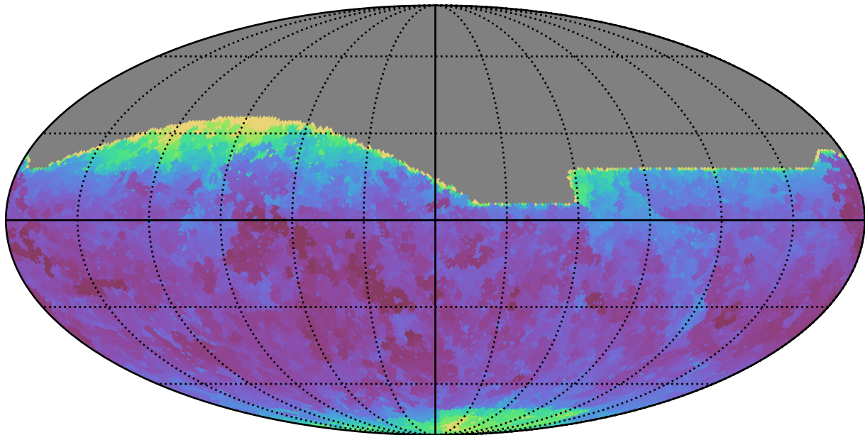
baseline_v2.1_10yrs All sky i band: Min seeingEff
