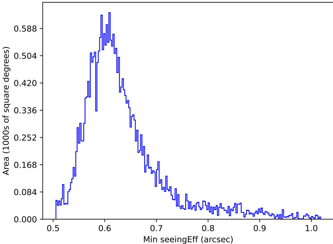
baseline_v2.1_10yrs All sky i band: Min seeingEff
