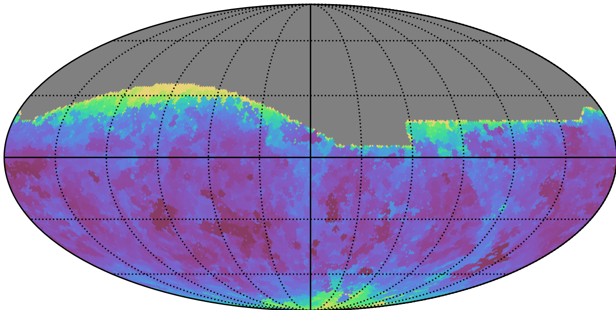
baseline_v2.1_10yrs All sky g band: Min seeingEff
