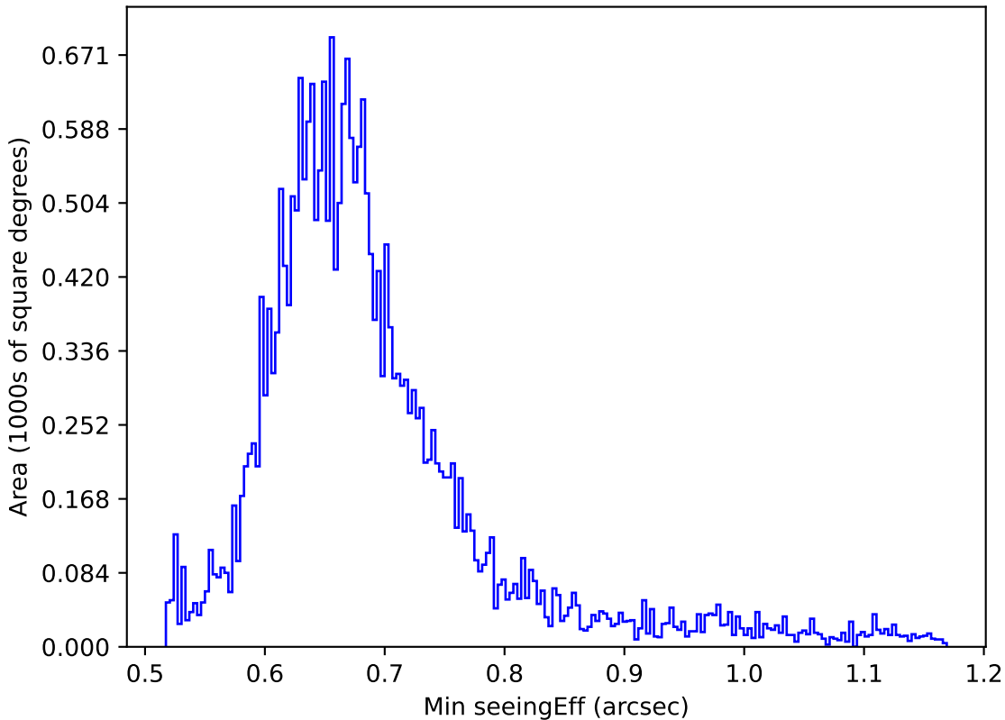
baseline_v2.1_10yrs All sky g band: Min seeingEff
