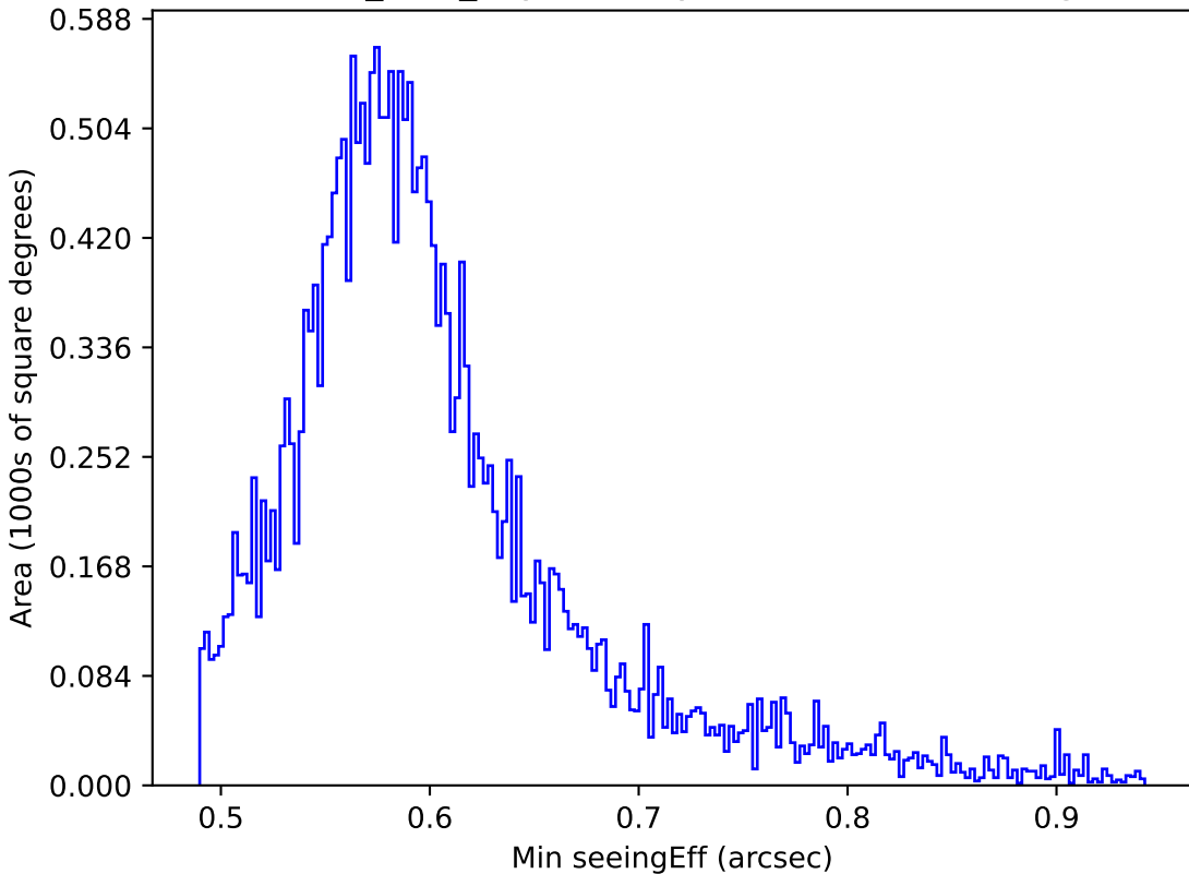
baseline_v2.1_10yrs All sky all bands: Min seeingEff
