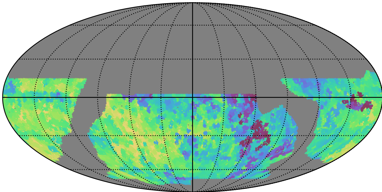
baseline_v2.1_10yrs WFD z band: Min saturation_mag
