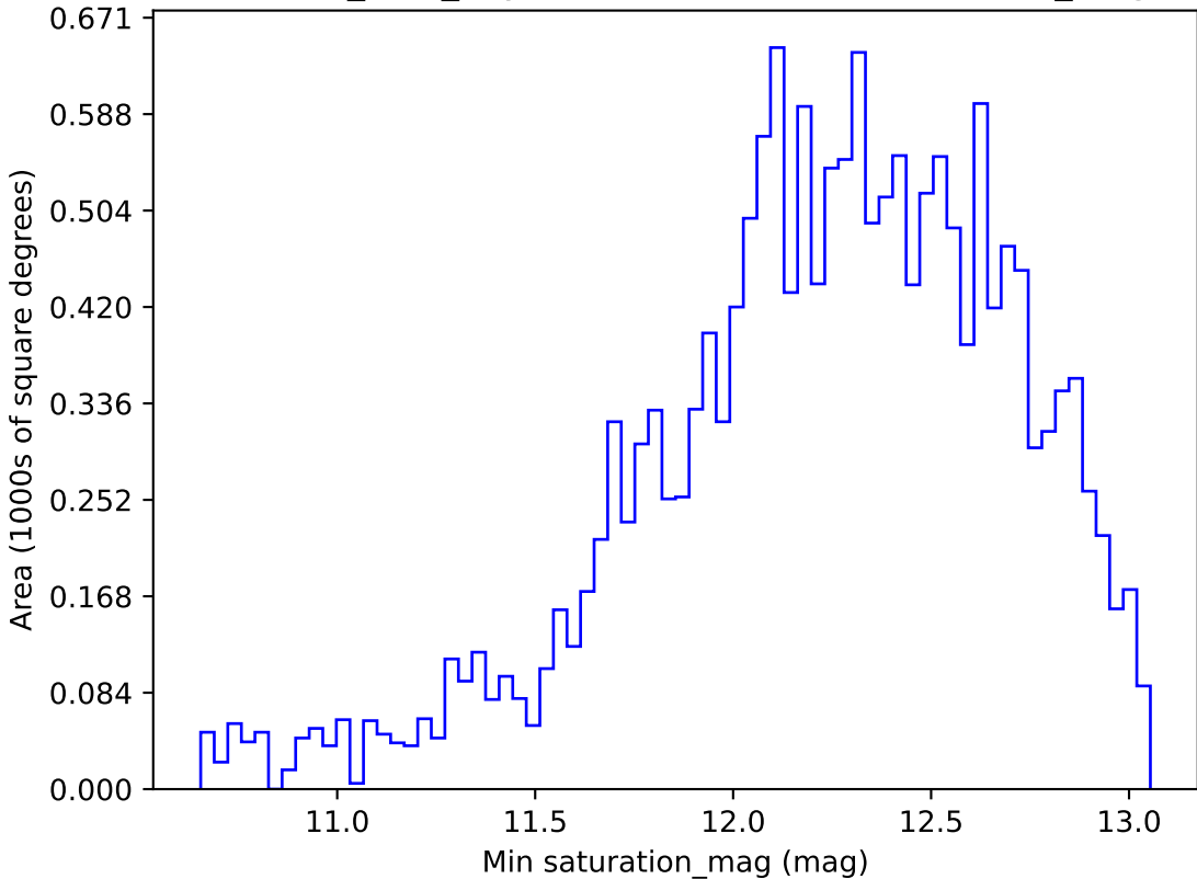
baseline_v2.1_10yrs WFD z band: Min saturation_mag
