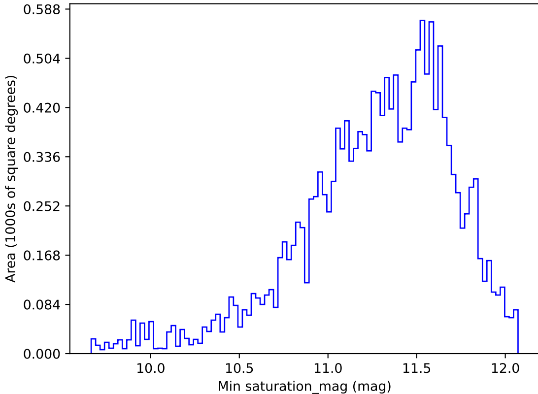
baseline_v2.1_10yrs WFD y band: Min saturation_mag
