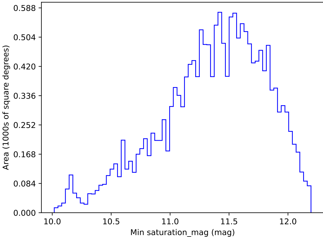
baseline_v2.1_10yrs WFD u band: Min saturation_mag
