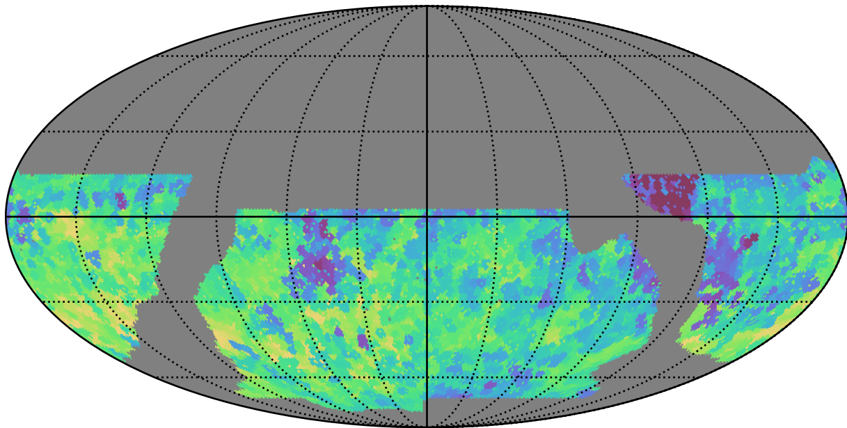
baseline_v2.1_10yrs WFD r band: Min saturation_mag
