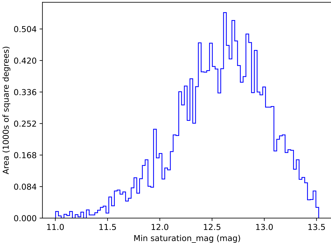
baseline_v2.1_10yrs WFD r band: Min saturation_mag
