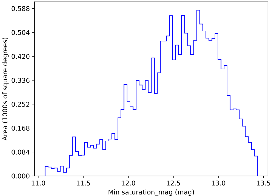
baseline_v2.1_10yrs WFD i band: Min saturation_mag
