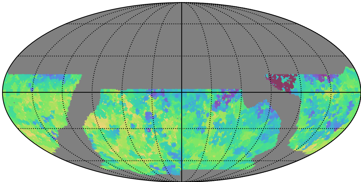
baseline_v2.1_10yrs WFD g band: Min saturation_mag
