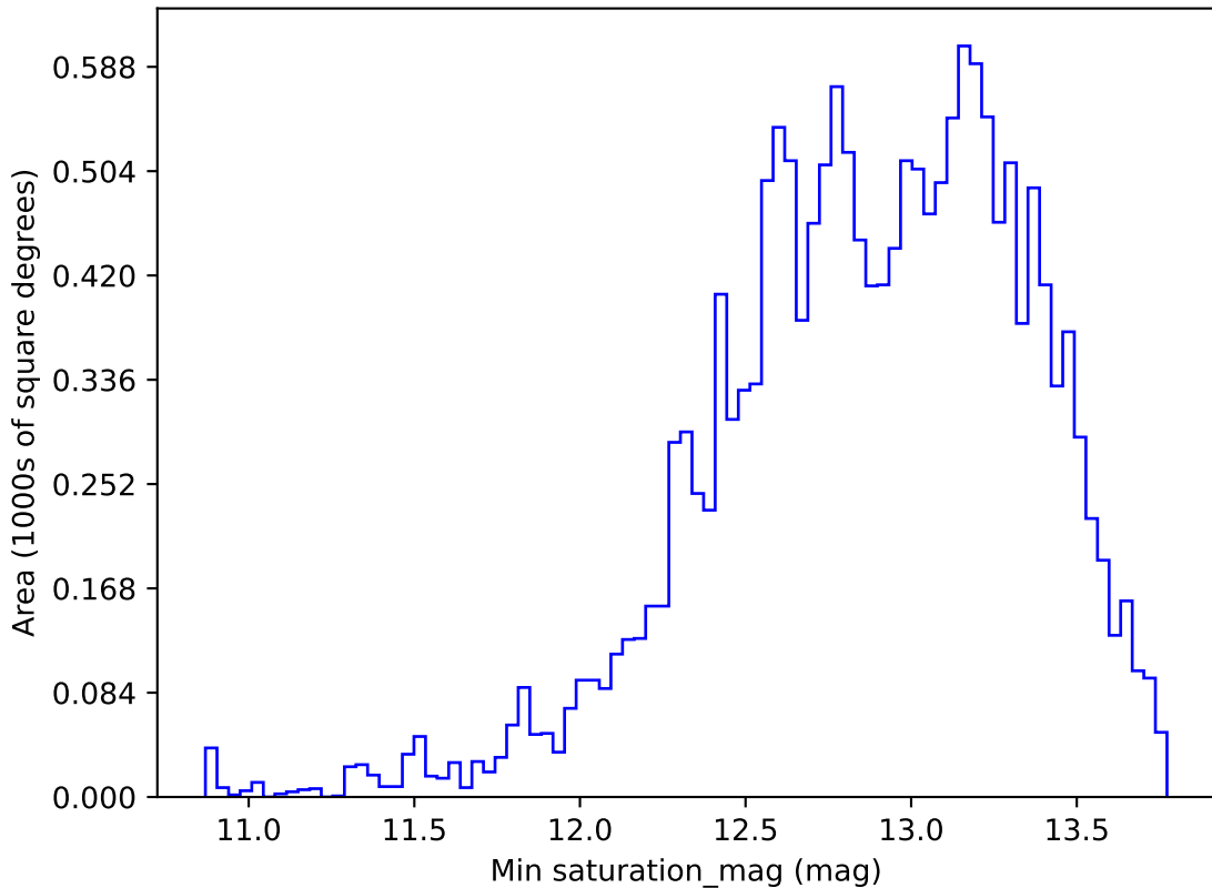
baseline_v2.1_10yrs WFD g band: Min saturation_mag
