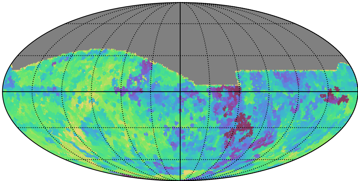
baseline_v2.1_10yrs All sky z band: Min saturation_mag
