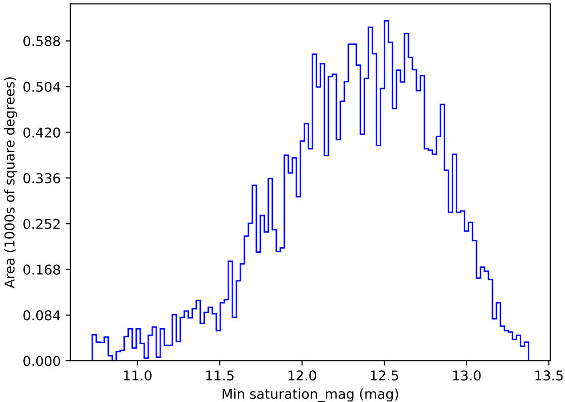
baseline_v2.1_10yrs All sky z band: Min saturation_mag
