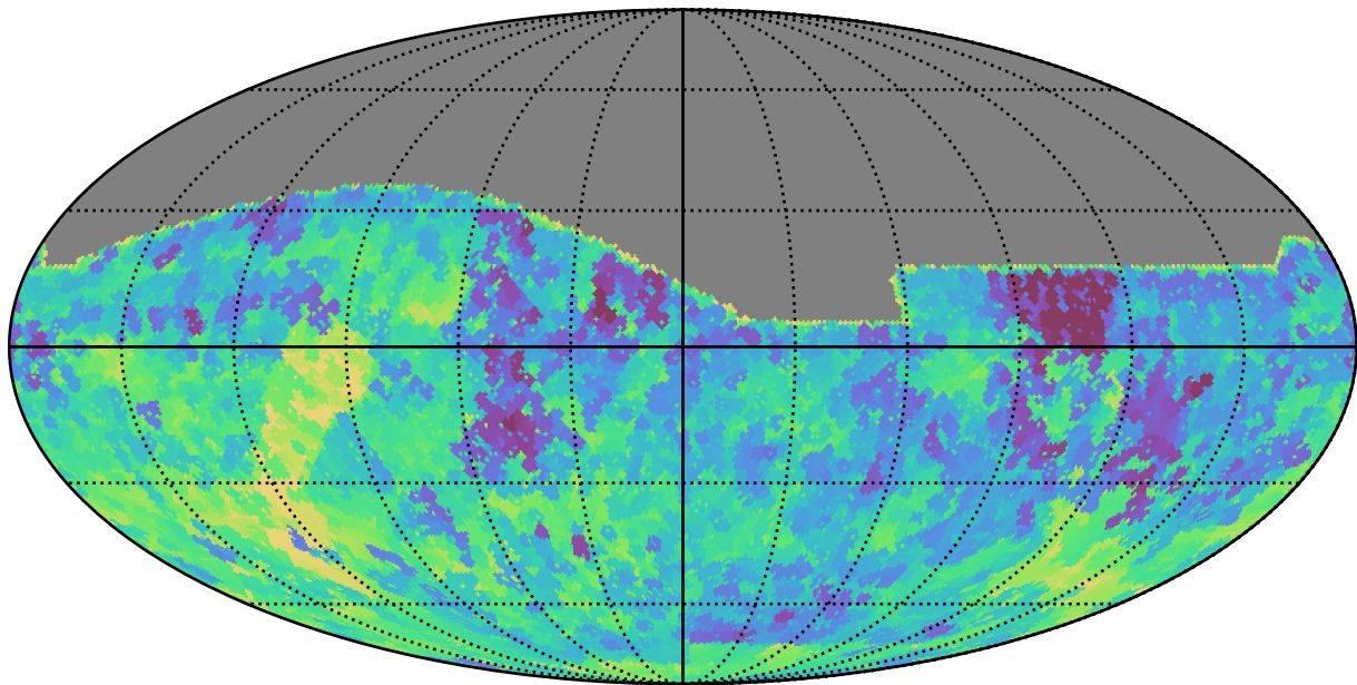
baseline_v2.1_10yrs All sky r band: Min saturation_mag
