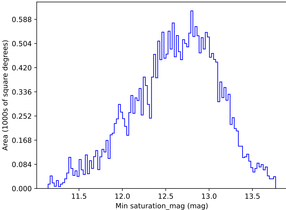
baseline_v2.1_10yrs All sky i band: Min saturation_mag
