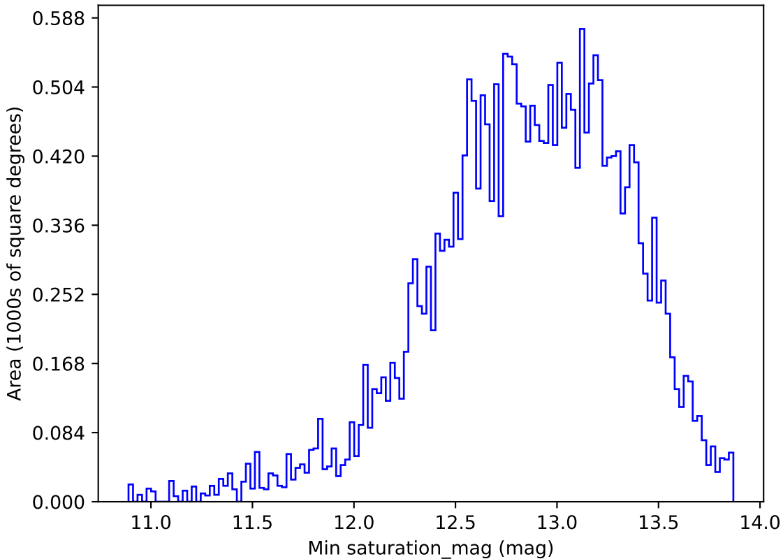
baseline_v2.1_10yrs All sky g band: Min saturation_mag
