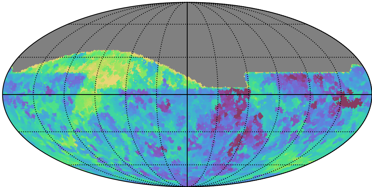
baseline_v2.1_10yrs All sky all bands: Min saturation_mag
