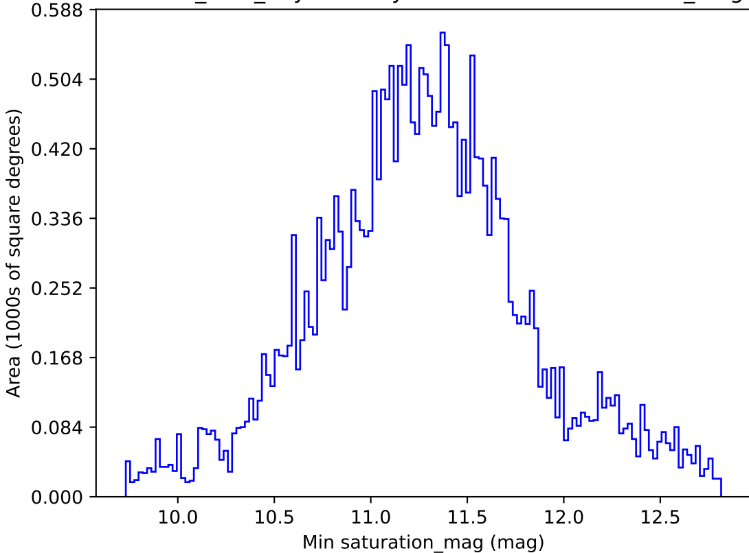
baseline_v2.1_10yrs All sky all bands: Min saturation_mag
