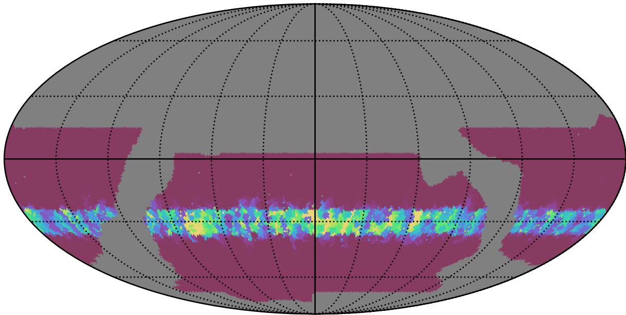
baseline_v2.1_10yrs WFD z band: Min normairmass
