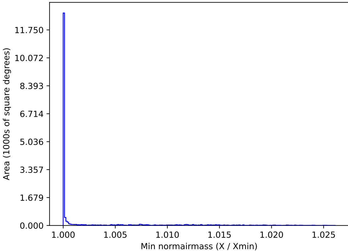
baseline_v2.1_10yrs WFD z band: Min normairmass
