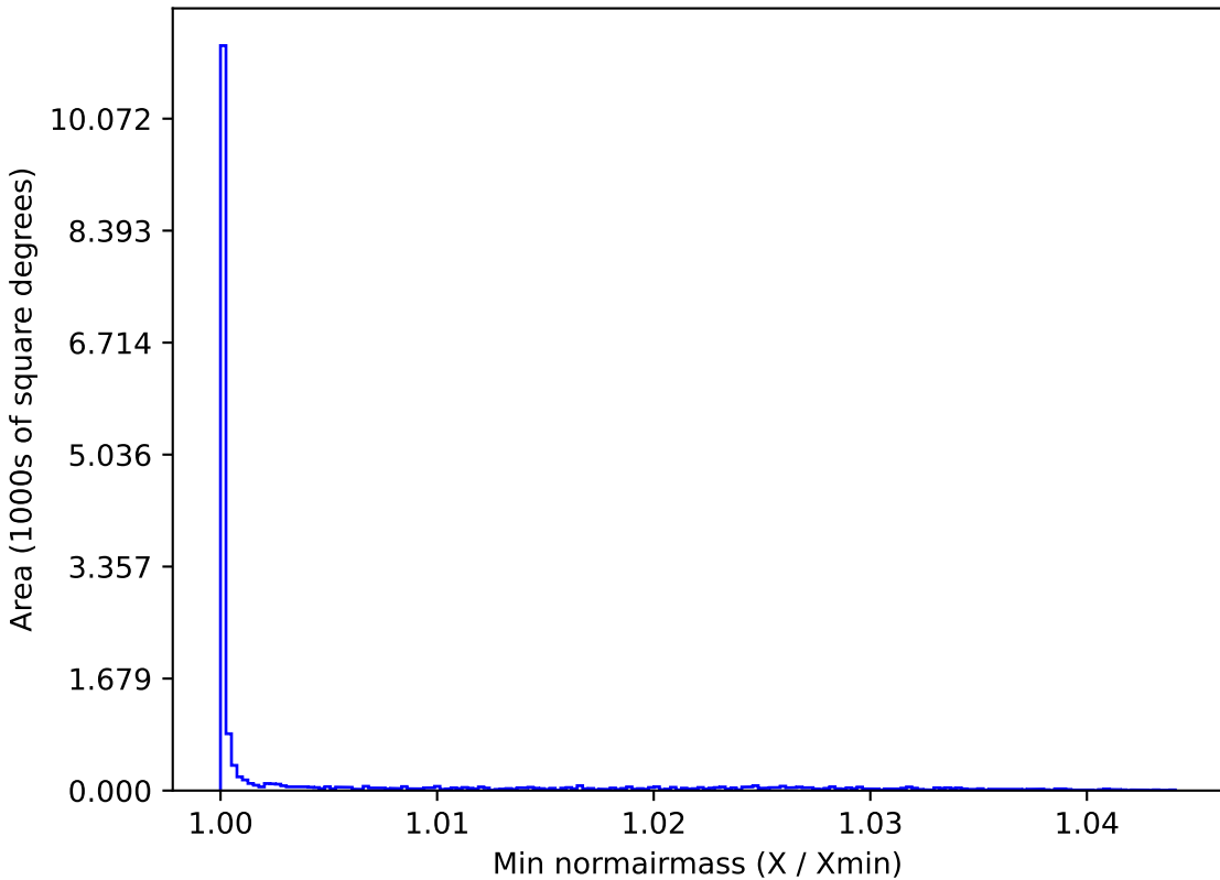
baseline_v2.1_10yrs WFD u band: Min normairmass
