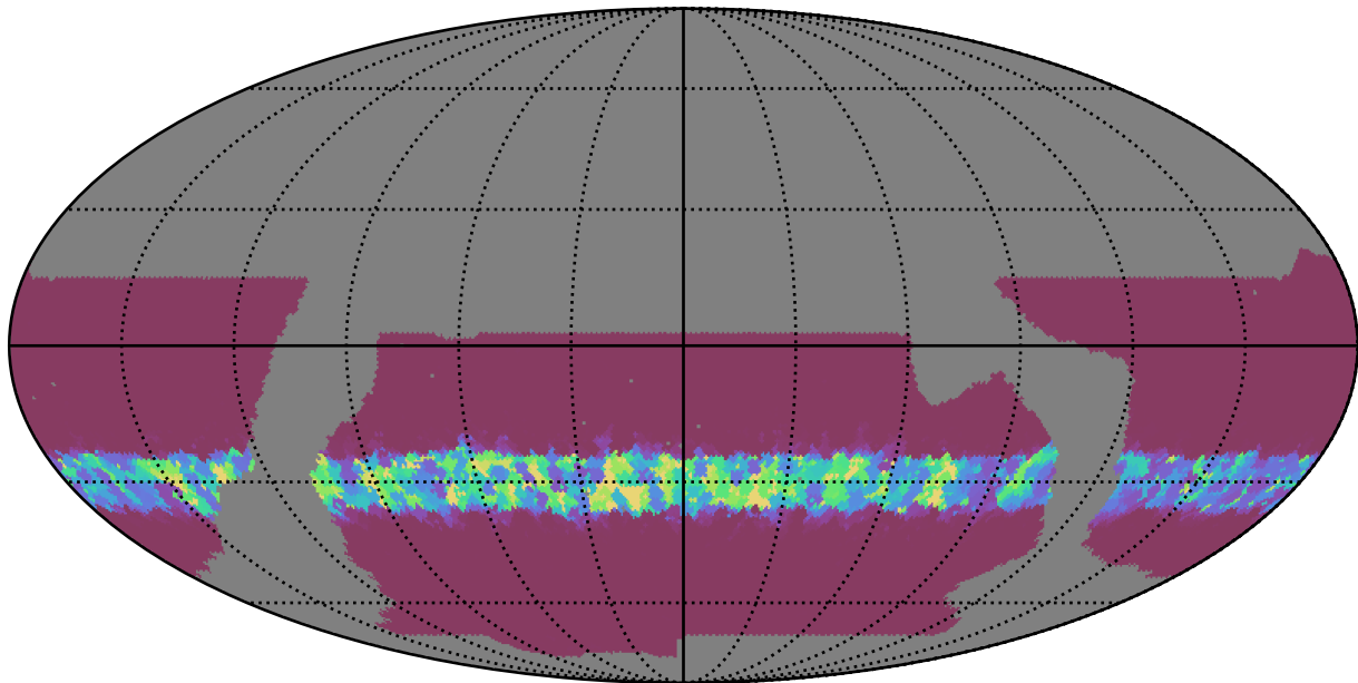
baseline_v2.1_10yrs WFD r band: Min normairmass
