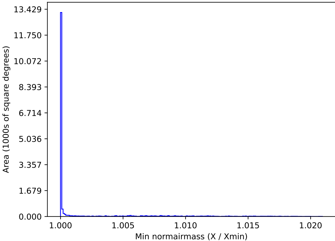
baseline_v2.1_10yrs WFD r band: Min normairmass
