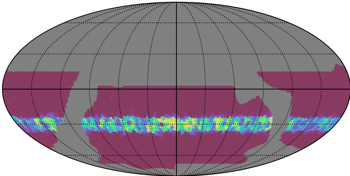
baseline_v2.1_10yrs WFD i band: Min normairmass
