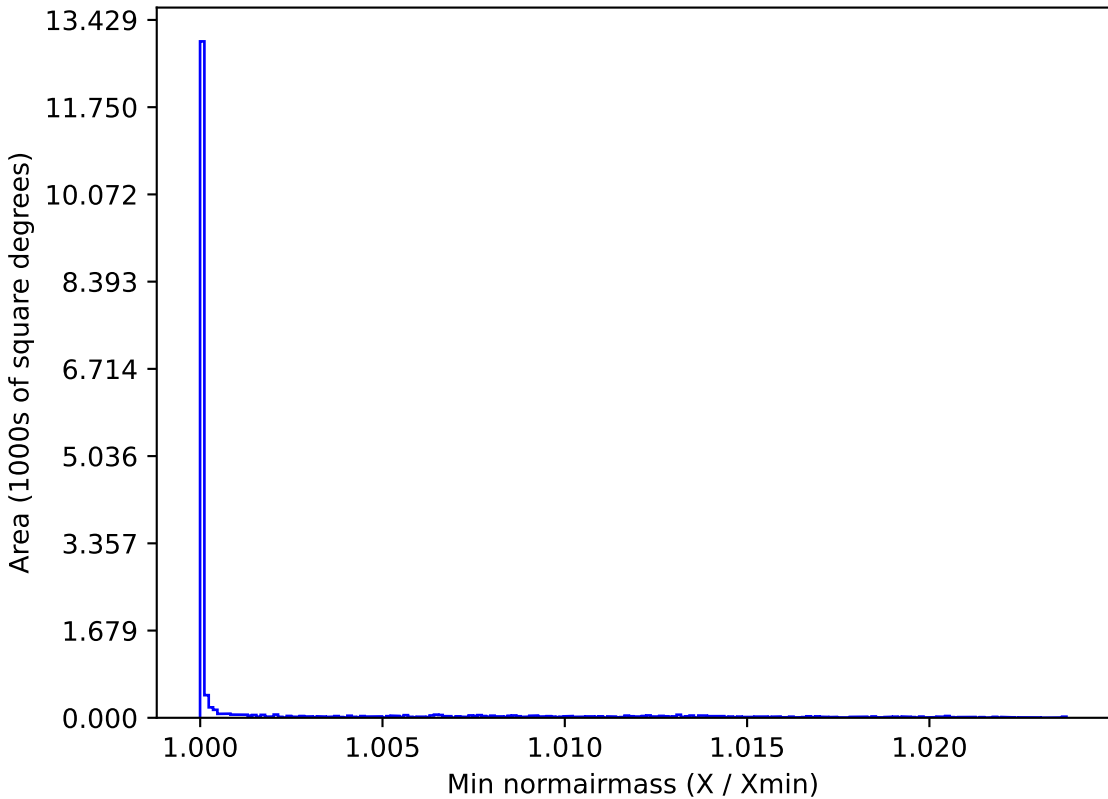
baseline_v2.1_10yrs WFD i band: Min normairmass
