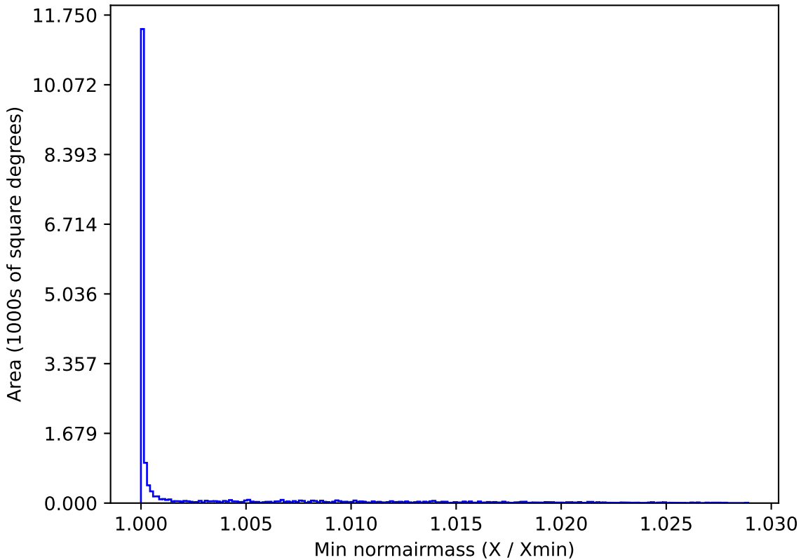
baseline_v2.1_10yrs WFD g band: Min normairmass
