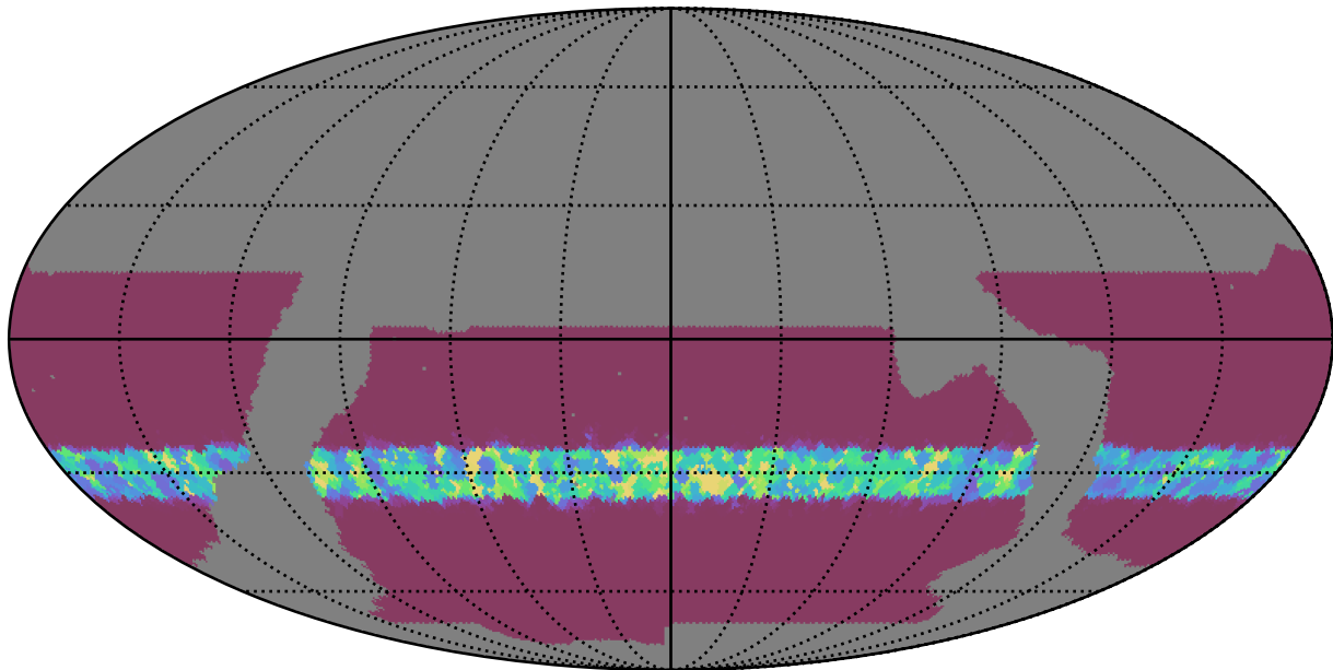
baseline_v2.1_10yrs WFD all bands: Min normairmass
