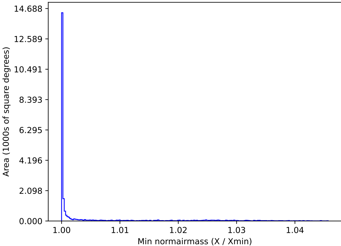
baseline_v2.1_10yrs All sky u band: Min normairmass
