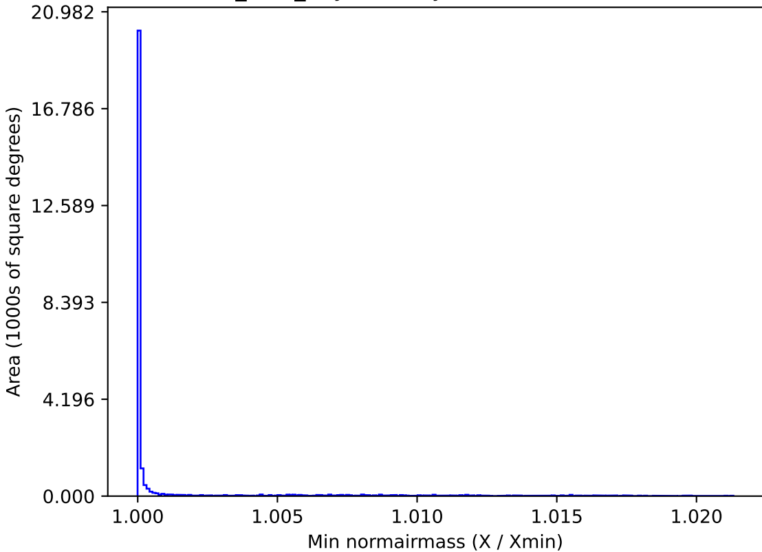
baseline_v2.1_10yrs All sky r band: Min normairmass
