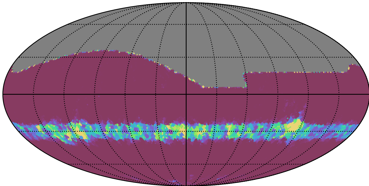
baseline_v2.1_10yrs All sky i band: Min normairmass
