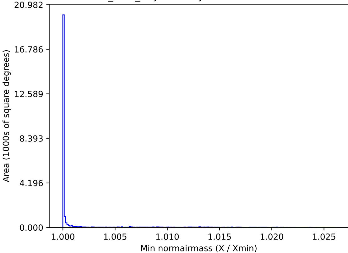
baseline_v2.1_10yrs All sky i band: Min normairmass
