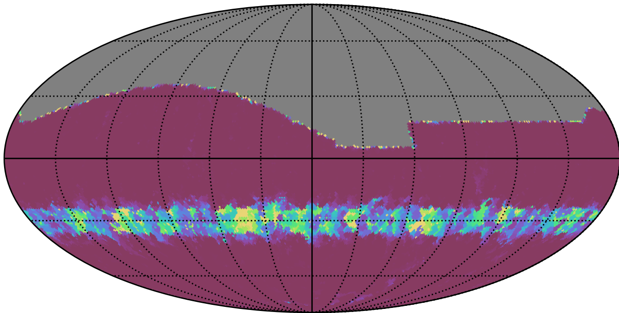
baseline_v2.1_10yrs All sky g band: Min normairmass
