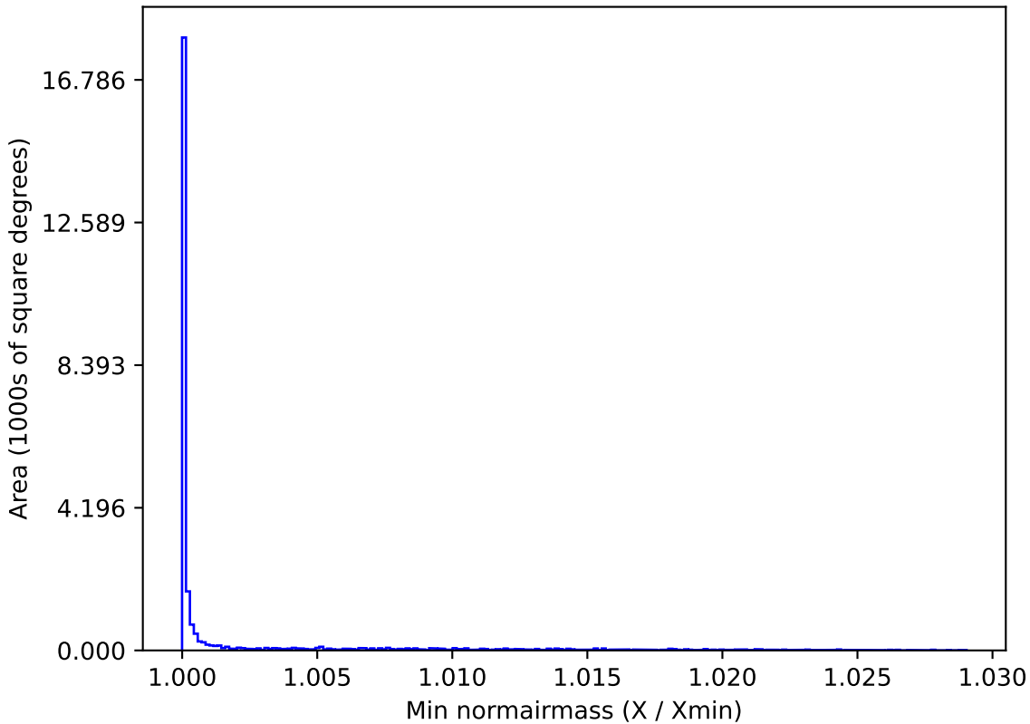
baseline_v2.1_10yrs All sky g band: Min normairmass
