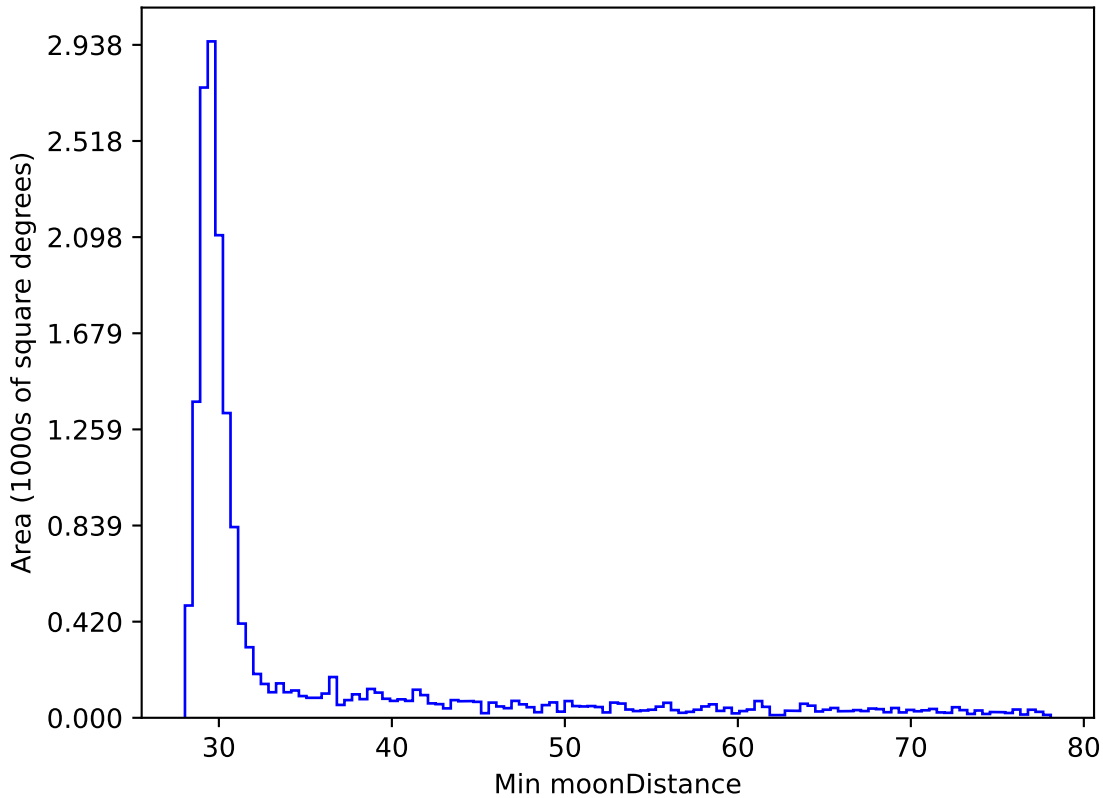
baseline_v2.1_10yrs WFD z band: Min moonDistance
