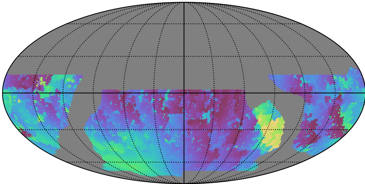
baseline_v2.1_10yrs WFD u band: Min moonDistance
