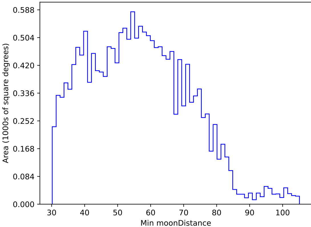
baseline_v2.1_10yrs WFD u band: Min moonDistance
