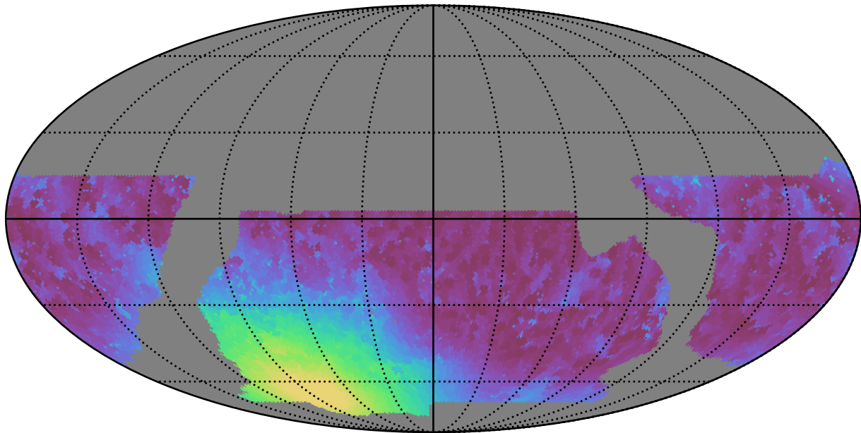
baseline_v2.1_10yrs WFD r band: Min moonDistance
