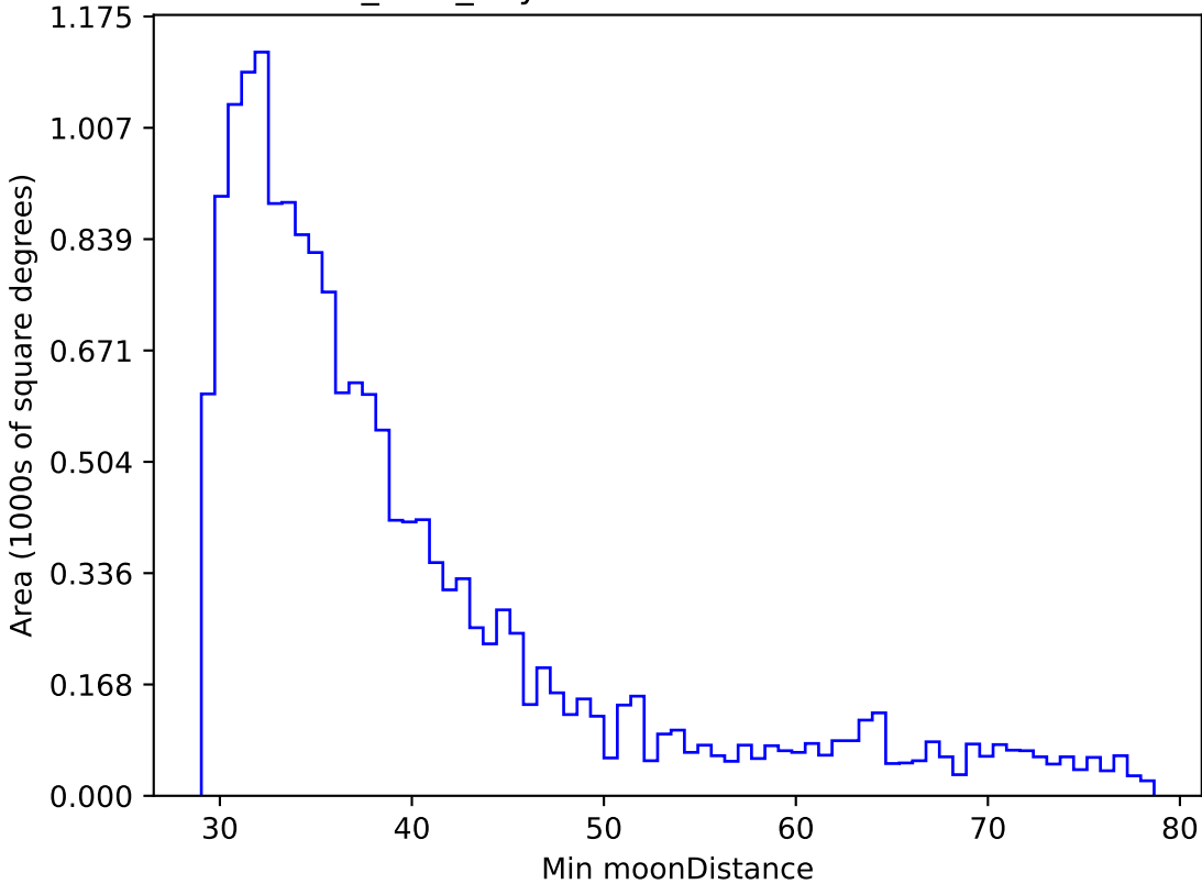
baseline_v2.1_10yrs WFD r band: Min moonDistance
