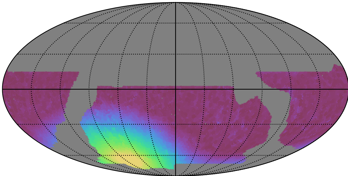
baseline_v2.1_10yrs WFD i band: Min moonDistance
