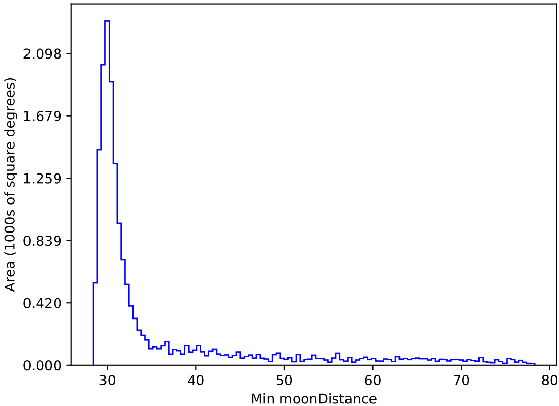
baseline_v2.1_10yrs WFD i band: Min moonDistance
