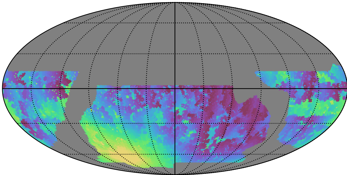
baseline_v2.1_10yrs WFD g band: Min moonDistance
