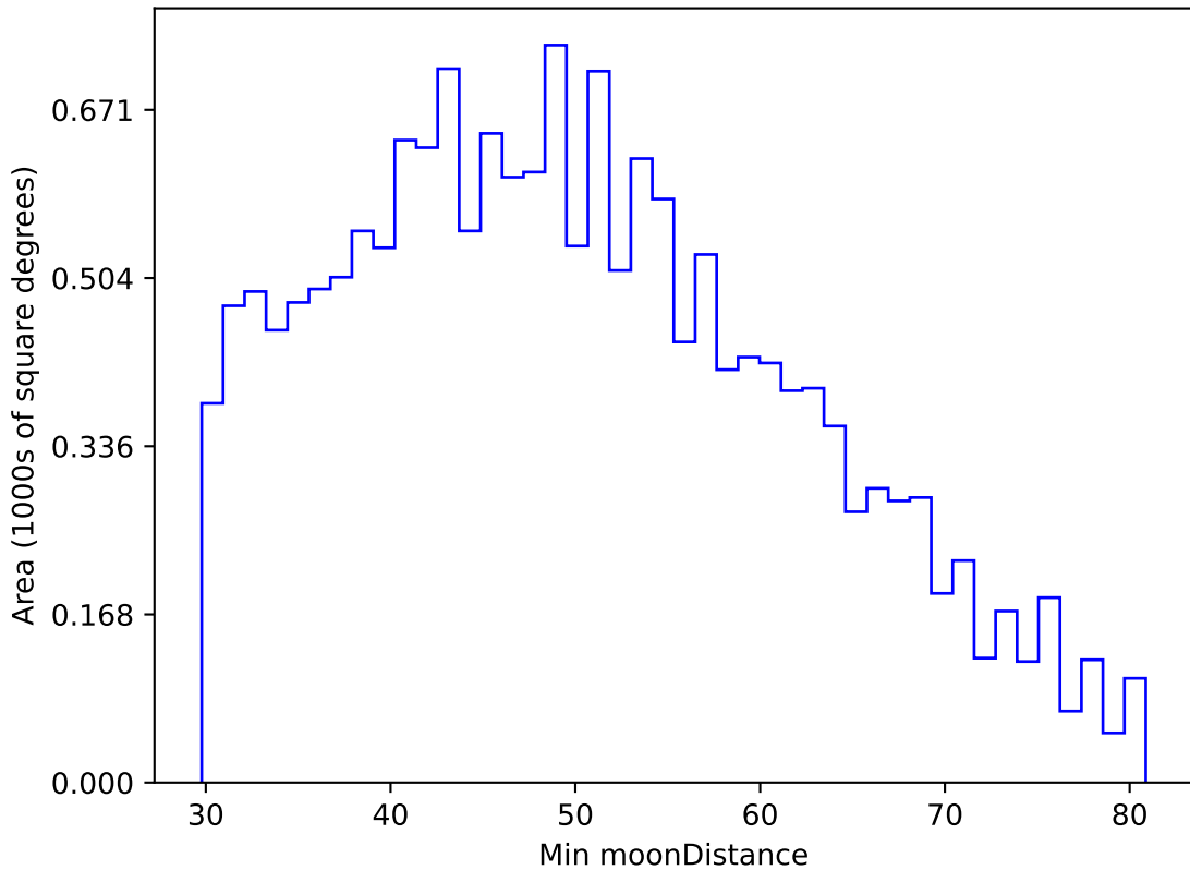
baseline_v2.1_10yrs WFD g band: Min moonDistance
