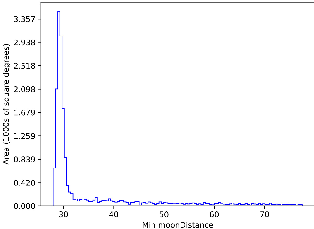
baseline_v2.1_10yrs WFD all bands: Min moonDistance
